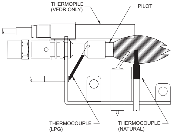
Correct Pilot Flame Pattern for VFDR Figure 21
