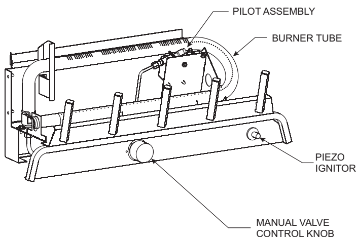
Thermostat Valve for VFDT Series Figure 18
