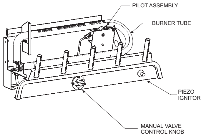
Manual Valve for VFDM Series Figure 19
