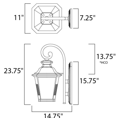
51127FSBZ Knoxville LED Outdoor Wall Lantern
