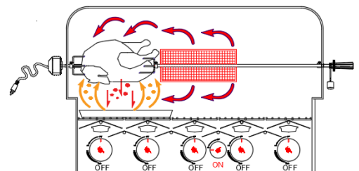
ROTISSERIE COOKING WITH INDIRECT HEAT USING INFRARED BACK BURNER ONLY
