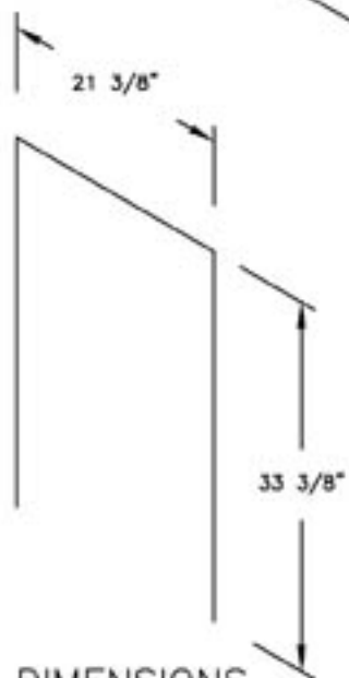
CUT-OUT DIMENSIONS
