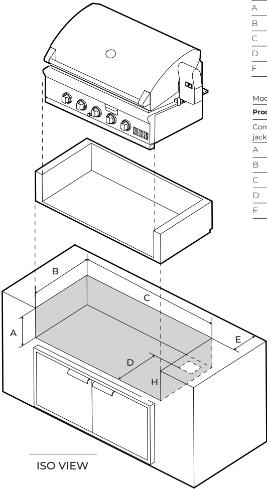
COMBUSTIBLE CABINET WITH INSULATION JACKET
