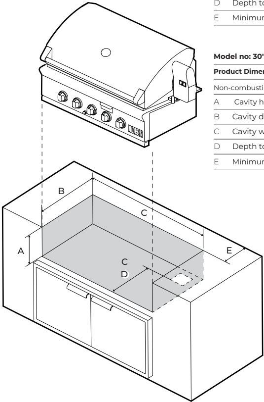
ISO VIEW
