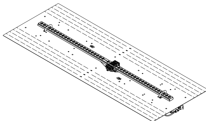
ISOMETRIC VIEW
