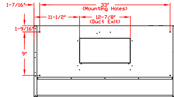
REAR VIEW (DUCT EXIT SHOWN IN BACK LOCATION)
