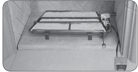
Fig. 20-1 Place sand/vermiculite
